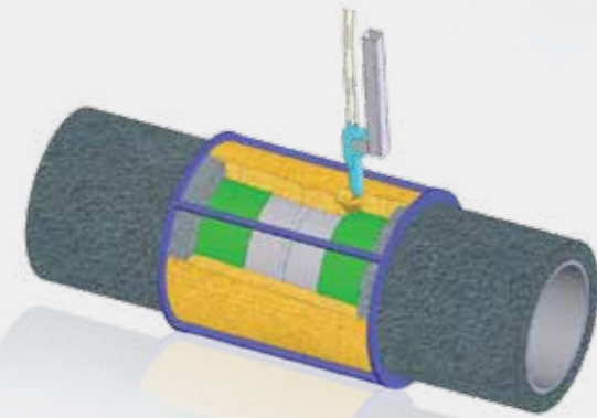
03. Solid polyurethane field joint.
