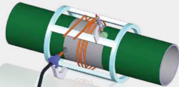
01. Fusion bonded epoxy field joint.
